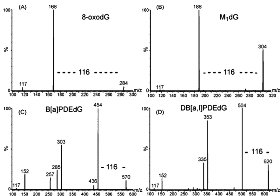
Figure 2. ESI MS/MS mass spectra documenting [M + H]^+ to [M + H - 116]^+ transitions of four DNA different adducts: (A) 8-oxo-dG, the main oxidative stress related DNA adduct; (B) M1dG, the main malondialdehyde adduct; (C) B[a]PDEdG, the main benzo[a]pyrene diol epoxide DNA adduct; and (D) DiB[a,l]PDEdG, a dibenzo[a,l]pyrene diol epoxide DNA adduct. Adapted from Farmer, P.B.; Singh, R. Mutat. Res.-Rev. Mutat. 2008 , 659, 68–76 (ref 13). Copyright 2008 Elsevier.
